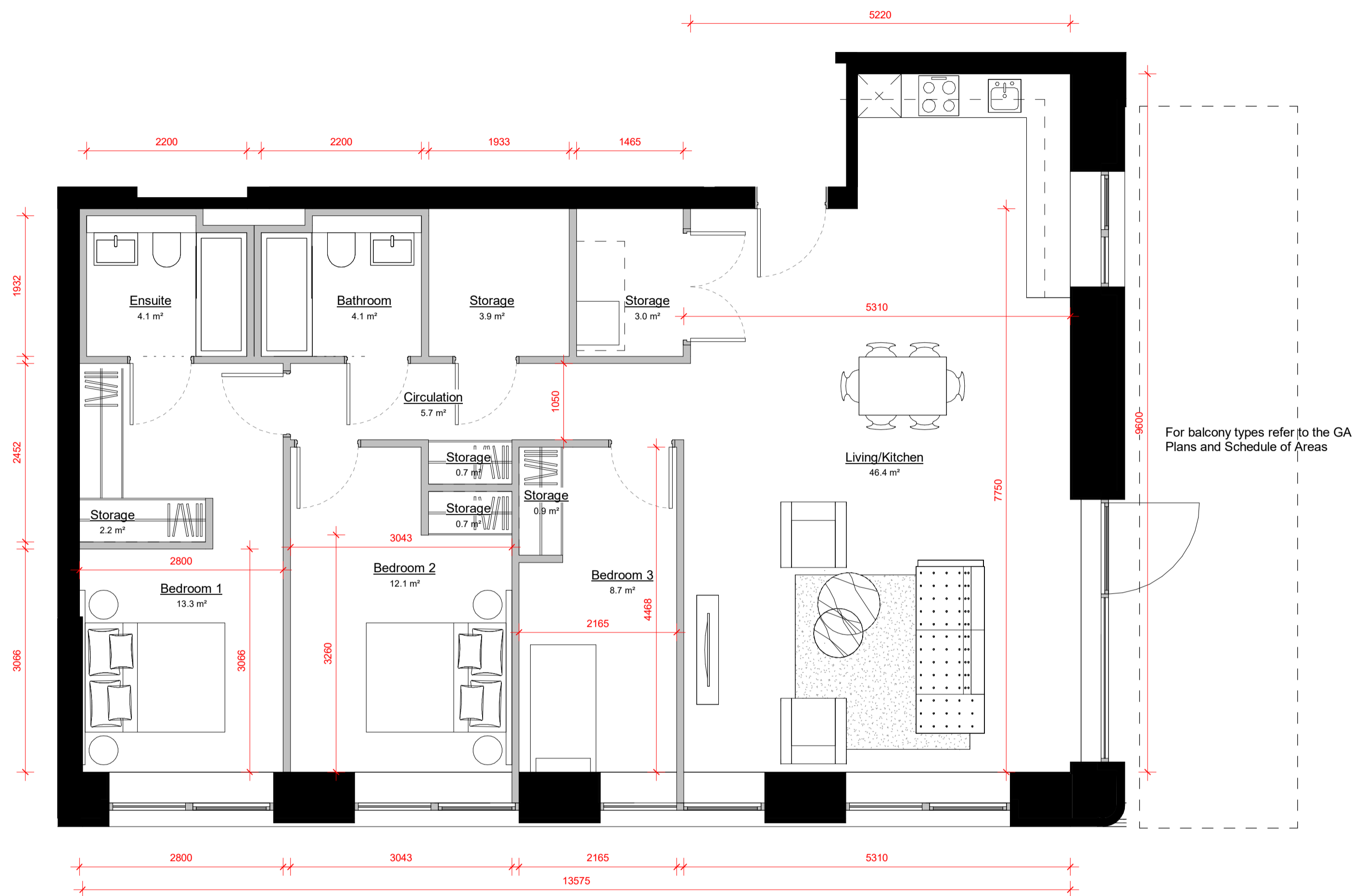
Apartment Type C.1.0 1 : 50
