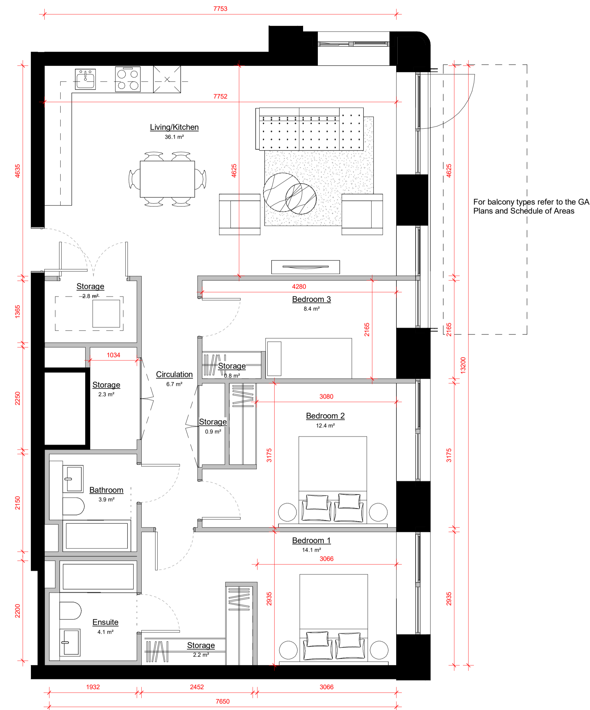
Apartment Type C.2.0 1 : 50
